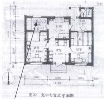
Suggested layout for a farm house.
